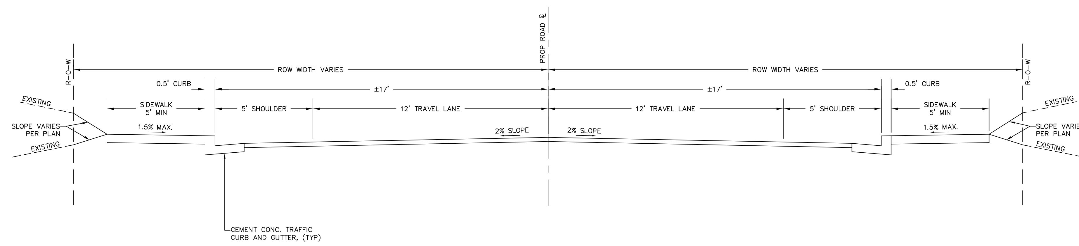
CROSS SECTION (TYP)
